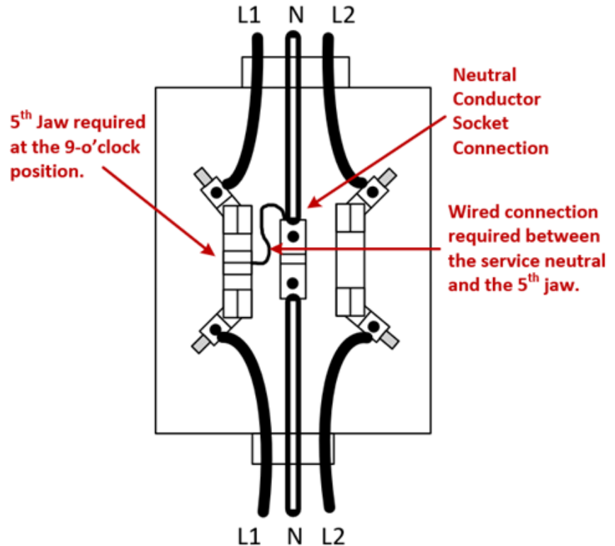
1-Phase, 3-wire, 120/208V Network Service Proper Meter Socket Connections
